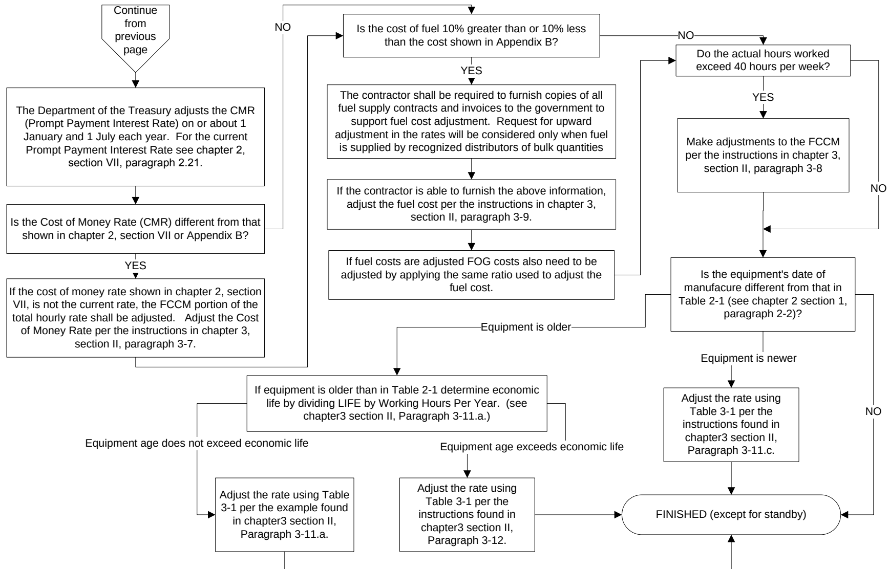
Figure 1-1. Methodology for Developing an Hourly Ownership and Operating Rate for Construction Equipment 1-4
