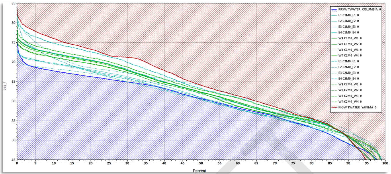
Figure 4-28. 15-April through 15-November Exceedance durations of provisional hindcast estimates for mixing temperature across sites W1-W4 and E1-E4 for Measure 7. Realized temperature benefits in the Yakima Delta fall within the unshaded plot area.
