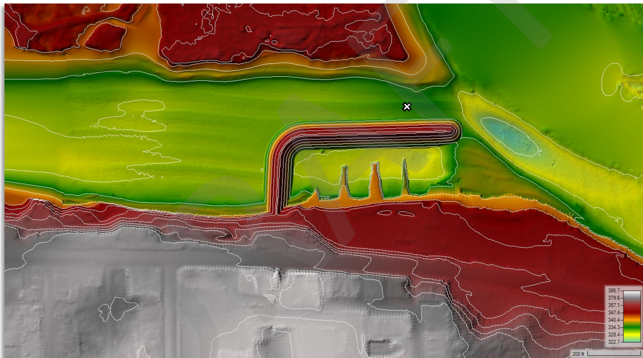
Figure 4-8. Layout for conceptual marina protection barrier levee M1 with velocity sampling location depicted.
