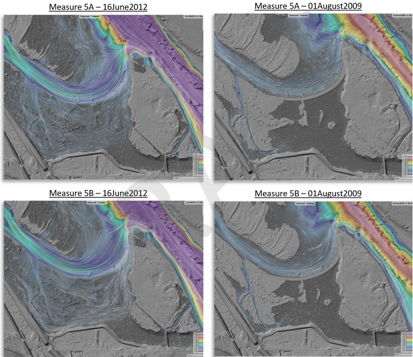
Figure 4-2. Overview of Measure 5 index velocity. Top: 5A, Bottom: 5B. Left: Spring Index - 16June2012, Right: Summer Index - 1Aug2009.
