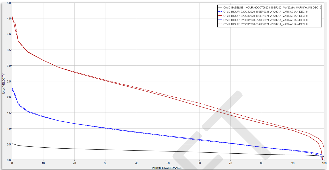
Figure 4-9. Exceedance duration of simulated velocity at the Marina causeway for Water Year 2021.
