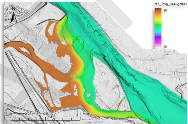
Figure 4-24. Measure7 (C1 – full causeway removal) simulation for late summer index conditions. (01Aug2009-High T, Low Q)
