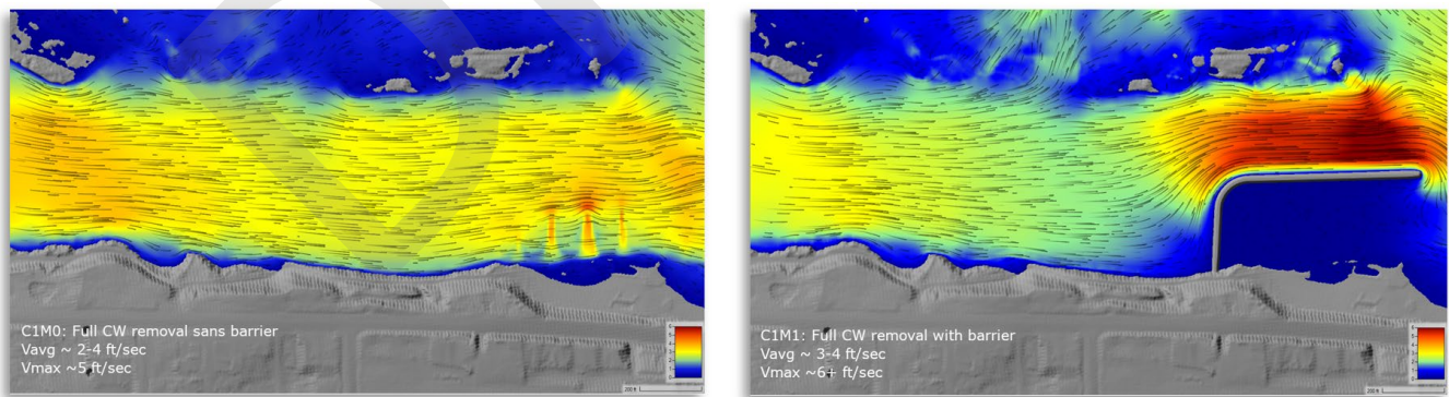
Figure 4-10. Simulated velocity for full causeway removal without (left) and with (right) marina barrier measure.
