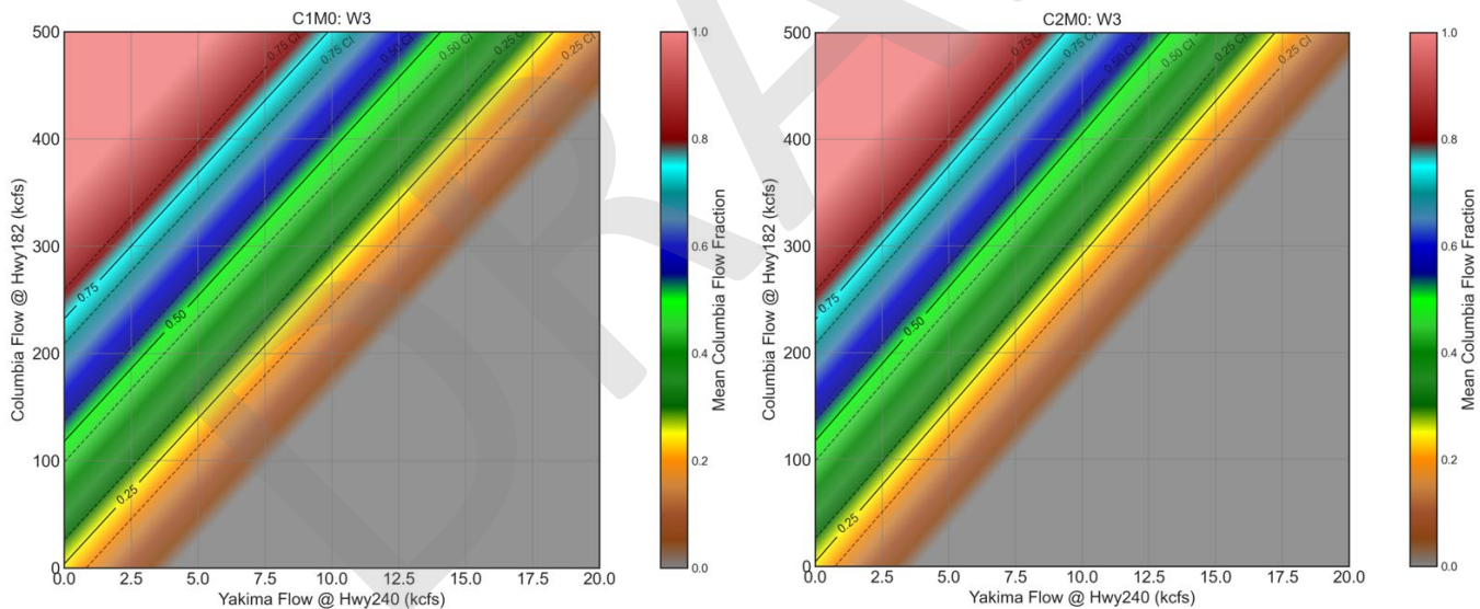
Figure 4-21. Provisional ratings with \alpha=0.05 for Columbia River flow fraction at Site W3. Left: Full causeway removal (C1M0), Right: Partial north causeway removal (C2M0).
