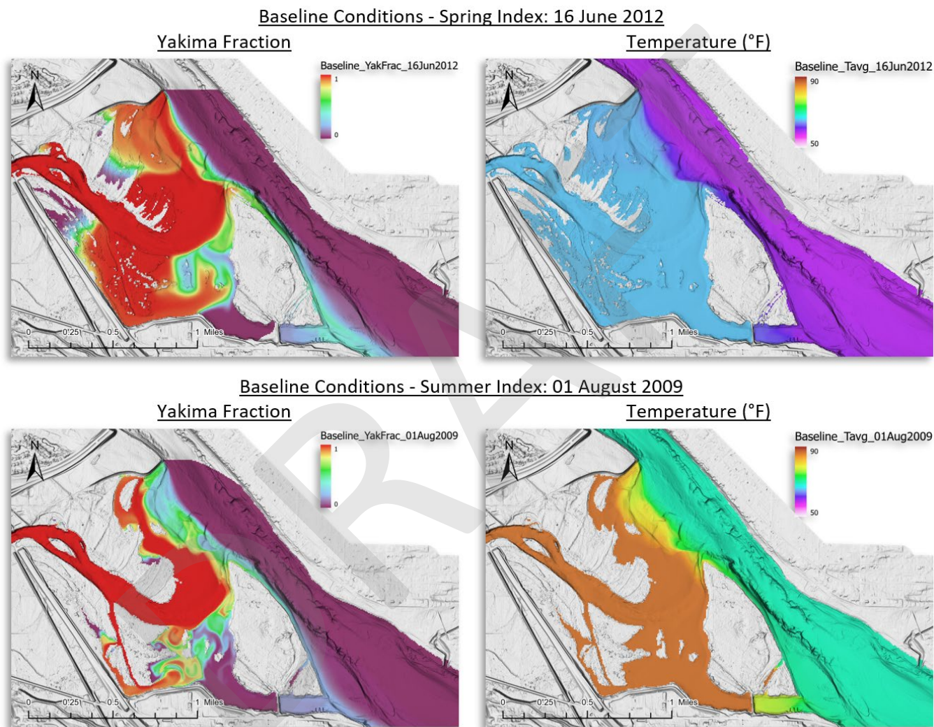
Figure 3-12. Baseline temperature simulation for late summer index conditions. (01Aug2009- High T, Low Q)
