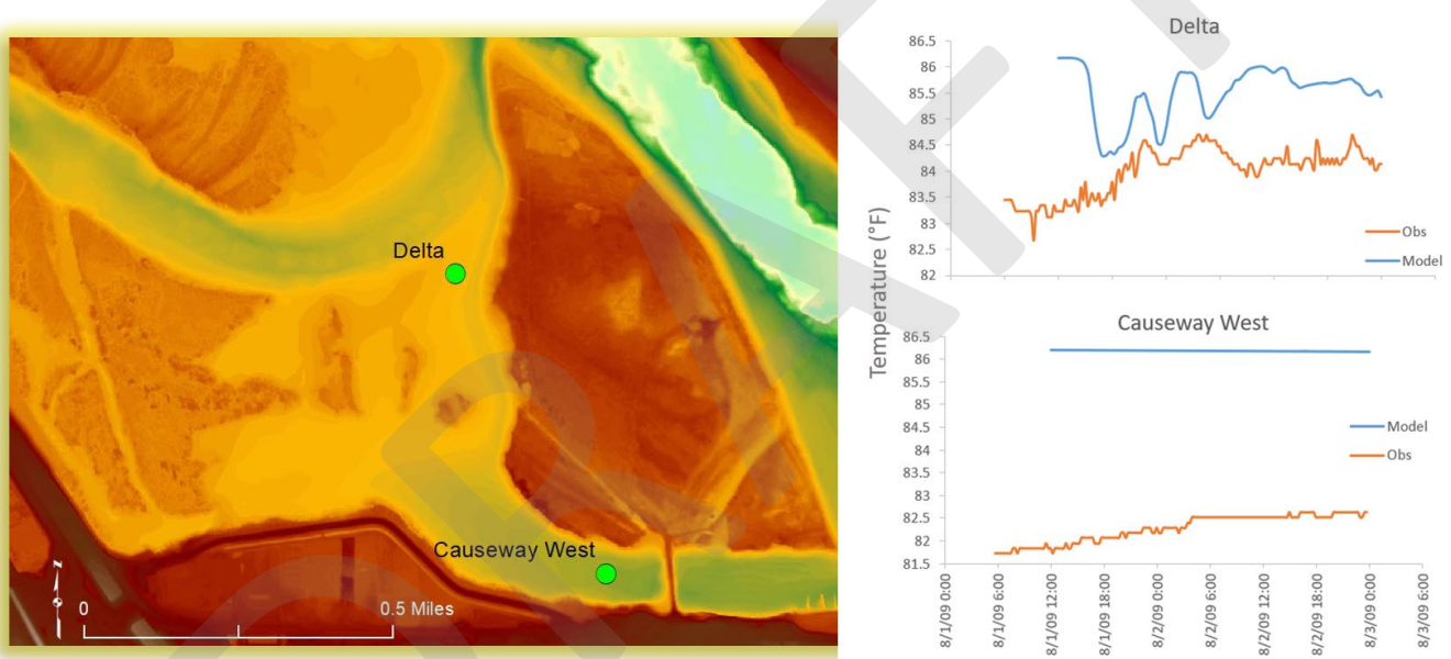
Figure 3-2. Historical Temperature Measurement Locations and initial Flow-3D model response.
