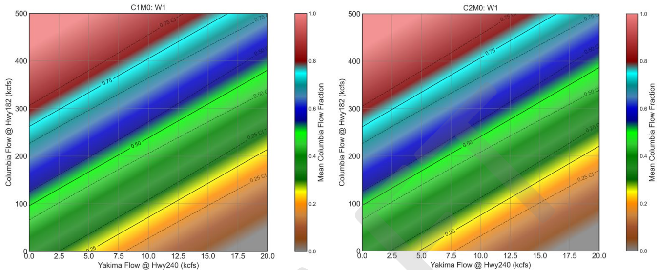
Figure 4-20. Provisional ratings with \alpha=0.05 for Columbia River flow fraction at Site W1 near the north end of Bateman Island. Left: Full causeway removal (C1M0), Right: Partial north causeway removal (C2M0).
