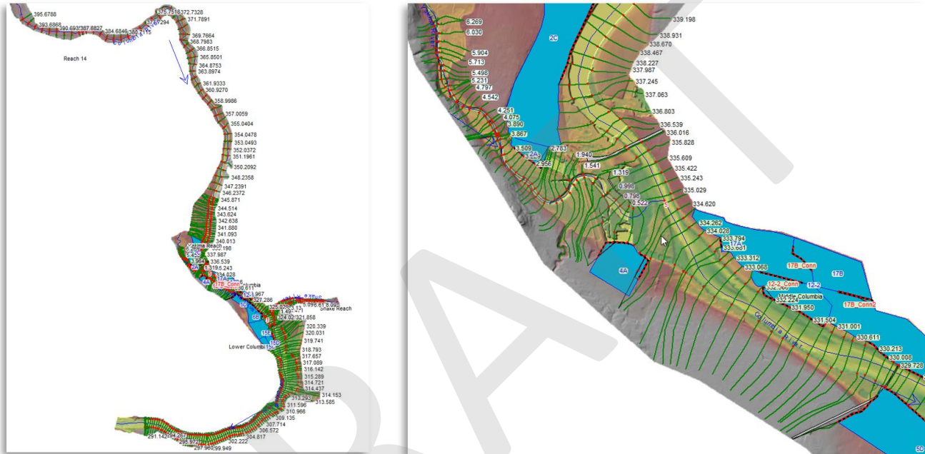
Figure 2-7. Regional HEC-RAS 1D model extents (left) and study area detail (right)
