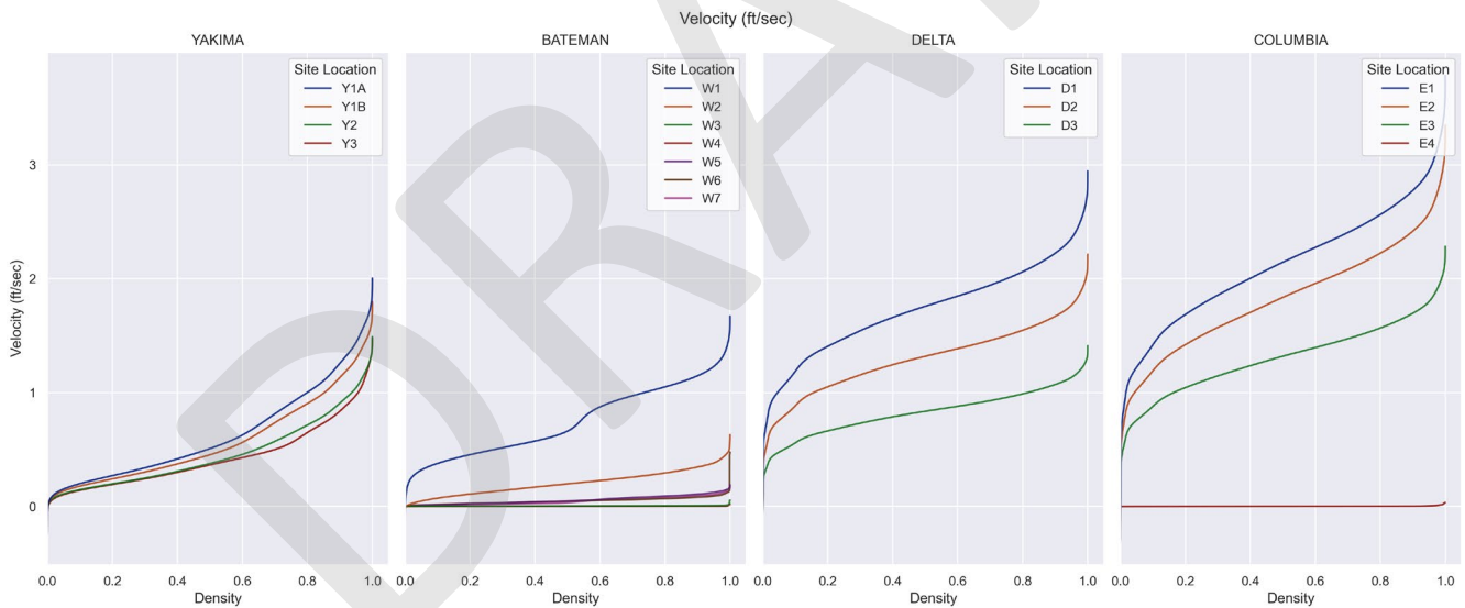
Figure 3-7. Cumulative distributions of modeled baseline velocity for May through September 2021 at select monitoring locations by sub-reach.
