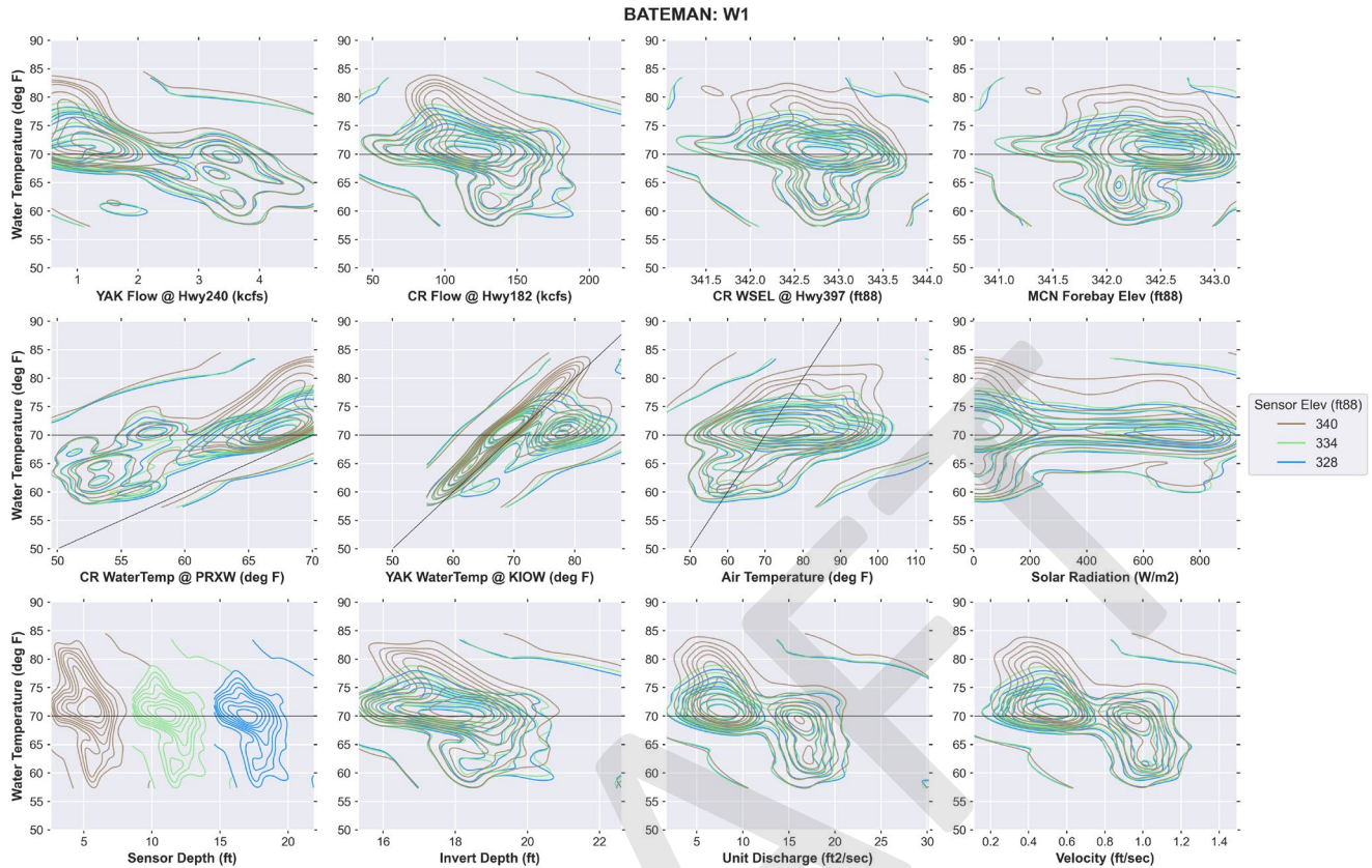
Figure 3-9. Kernel Density Estimate plots of measured summer 2021 water temperatures versus various exogenous parameters at site W1 on the Northwest Side of Bateman Island.
