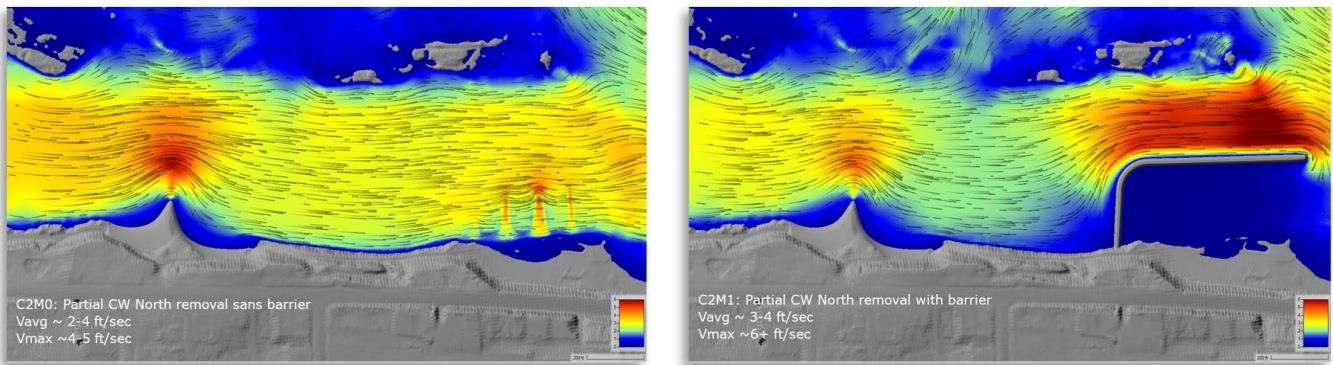
Figure 4-11. Simulated velocity for partial north causeway removal without (left) and with (right) marina levee barrier measure.
