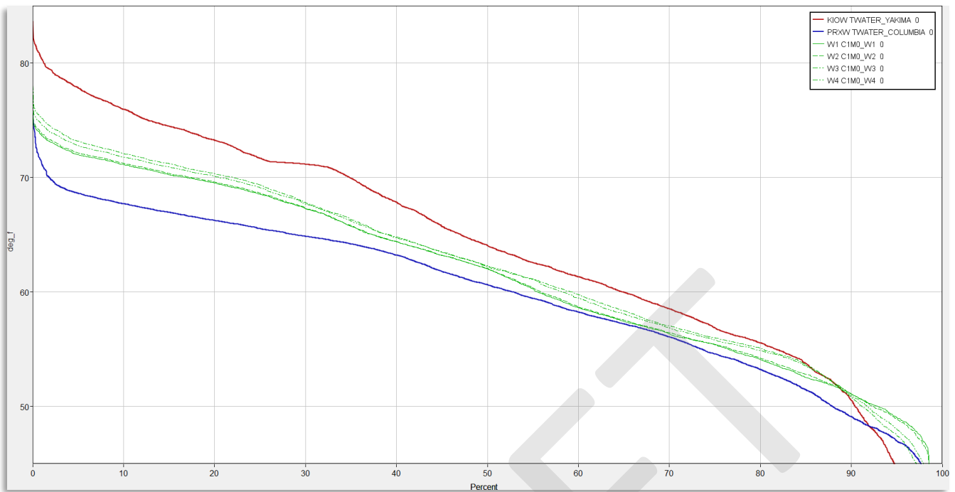
Figure 4-26. 15-April through 15-November Exceedance durations of provisional hindcast estimates for mixing temperature at sites W1 through W4 for Measure 7 with full causeway removal (C1M0).
