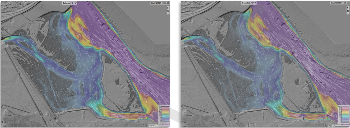
Figure 4-6. Measure 7 model simulation depicting unit discharge on 7June2021 from 0 to >30 cfs/ft. Left: full causeway removal (C1); Right: partial north causeway removal (C2).
