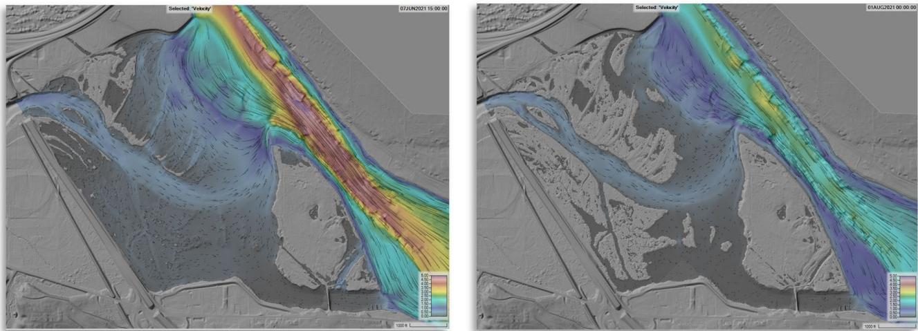
Figure 3-5. 2D model simulation depicting baseline velocity on 07June2021 (left) and 01Aug2021 (right). Note the relatively low baseline velocities southwest of Bateman Island.
