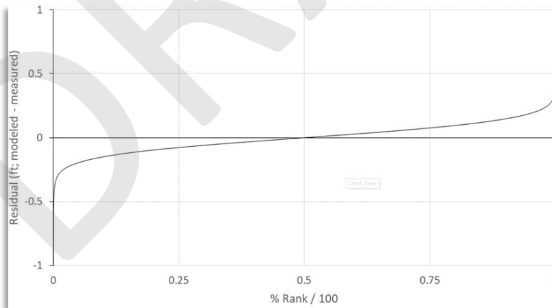
Figure 2-8. HEC-RAS 1D model residuals at Clover Island Gage (CCKW Gage#12514500)
