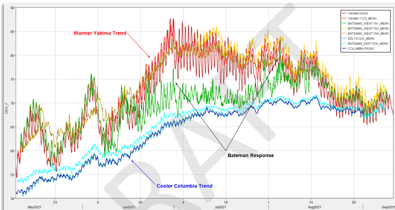
Figure 3-8. Timeseries of depth-averaged temperature string data measured between May and September 2021
