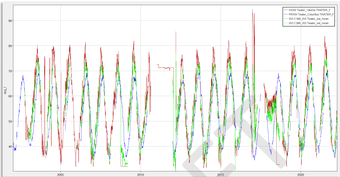
Figure 4-25. Timeseries of provisional hindcast estimates for mixing temperature at site W3 for WY 2004 to 2020.
