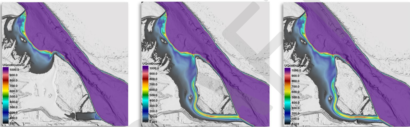
Figure 4-16. Simulated cumulative unit volume (acre-feet per foot) of Columbia River Water for March to September, 2021. Left: Baseline (C0M0), Center: Full Causeway Removal (C1M0), Right: Partial North Causeway Removal (C2M0). Note upper scale clipped to \geq 1 kaf/ft to highlight Yakima delta patterns.
