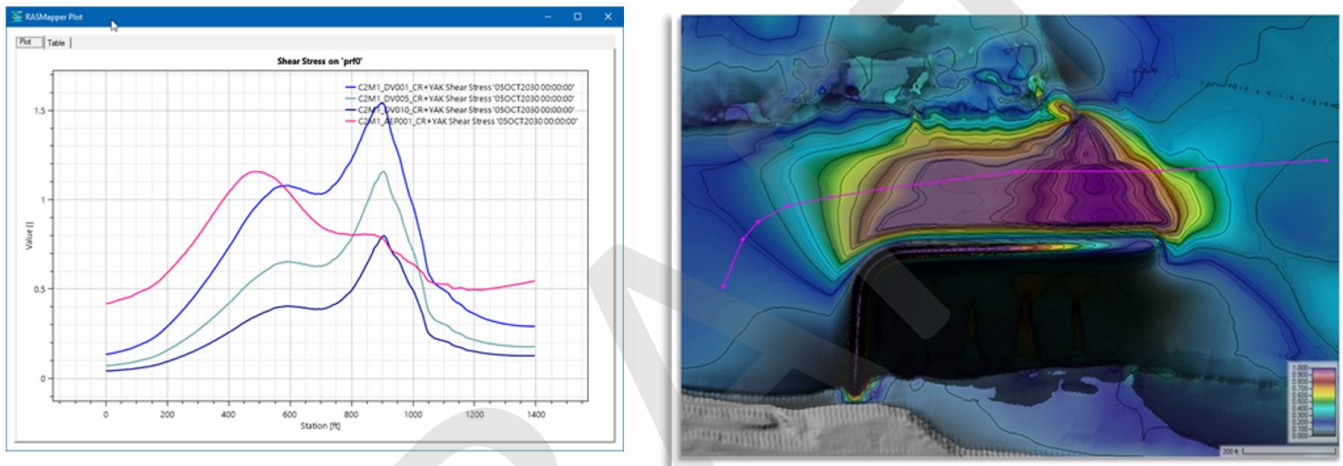
Figure 4-12. Shear Stress Profile along open causeway on North side of M1: Levee Marina Barrier
