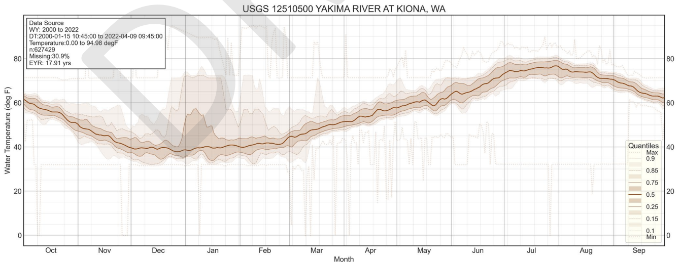
Figure 2-6. Daily quantiles for Yakima temperature at KLOW from water year 2000 to 2021.
