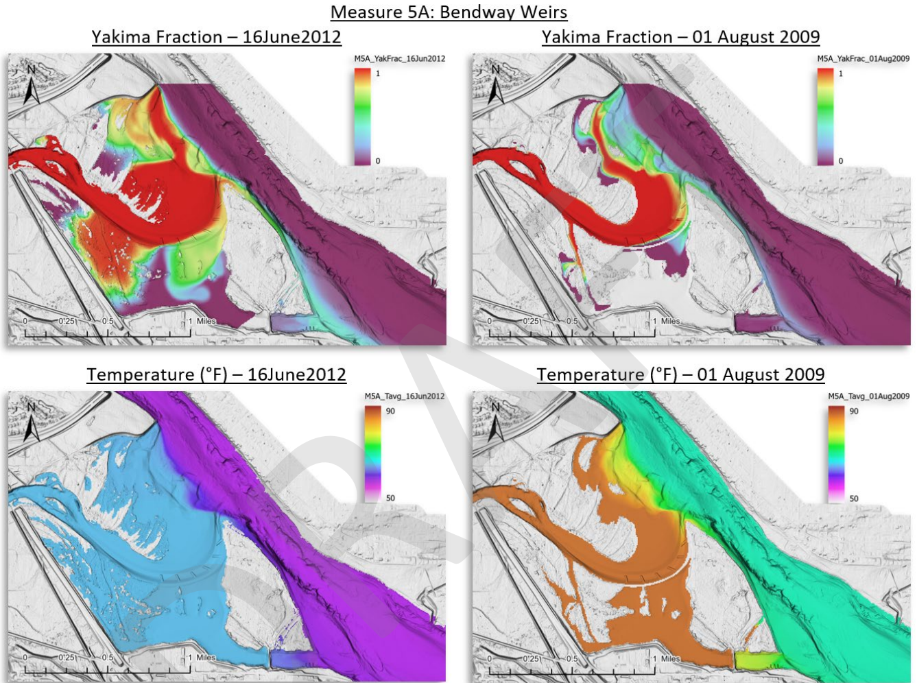
Figure 4-3. Overview of Measure 5A simulated index mixing fraction and temperature. Left: Spring Index - 16June2012. Right: Summer Index - 1Aug2009.
