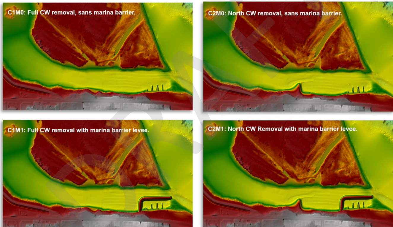
Figure 4-5. Overview of Measure 7 configuration geometries evaluated. Left: Full removal (C1); Right: Partial removal (C2); Bottom: with marina barrier levee (M1).
