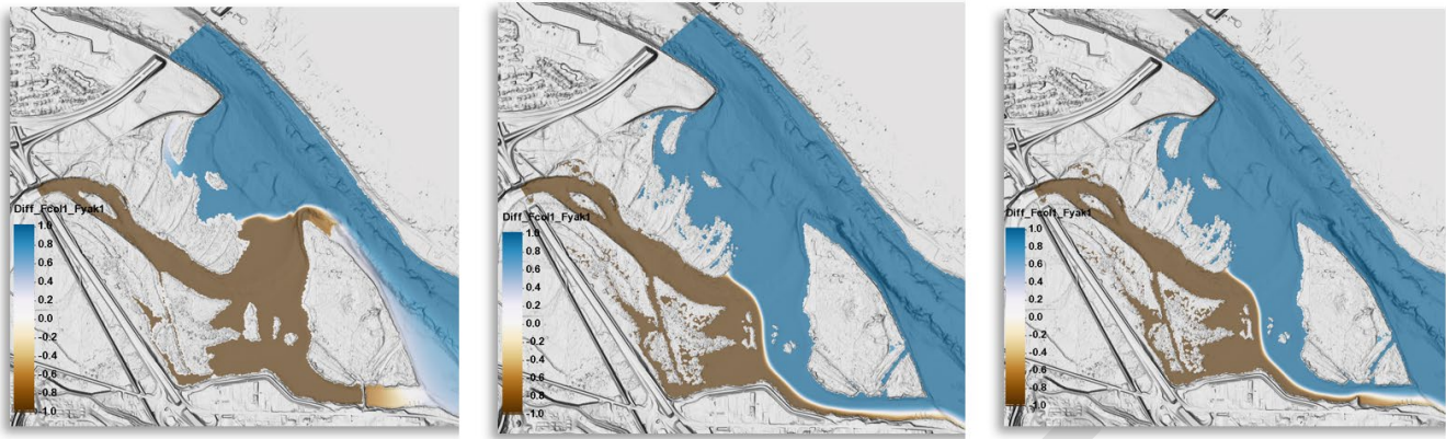
Figure 4-15. Simulations depicting mixing fractions of Columbia and Yakima River flows around Bateman Island on 28-June-2021. Left: Baseline (C0M0), Center: Full Causeway Removal (C1M0), Right: Partial North Causeway Removal (C2M0).
