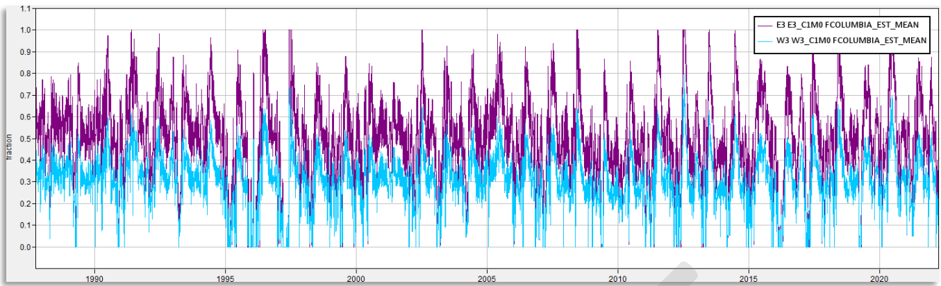
Figure 4-22. Timeseries of provisional hindcast for Columbia River flow fraction at site W3 for WY 1988 to 2020.
