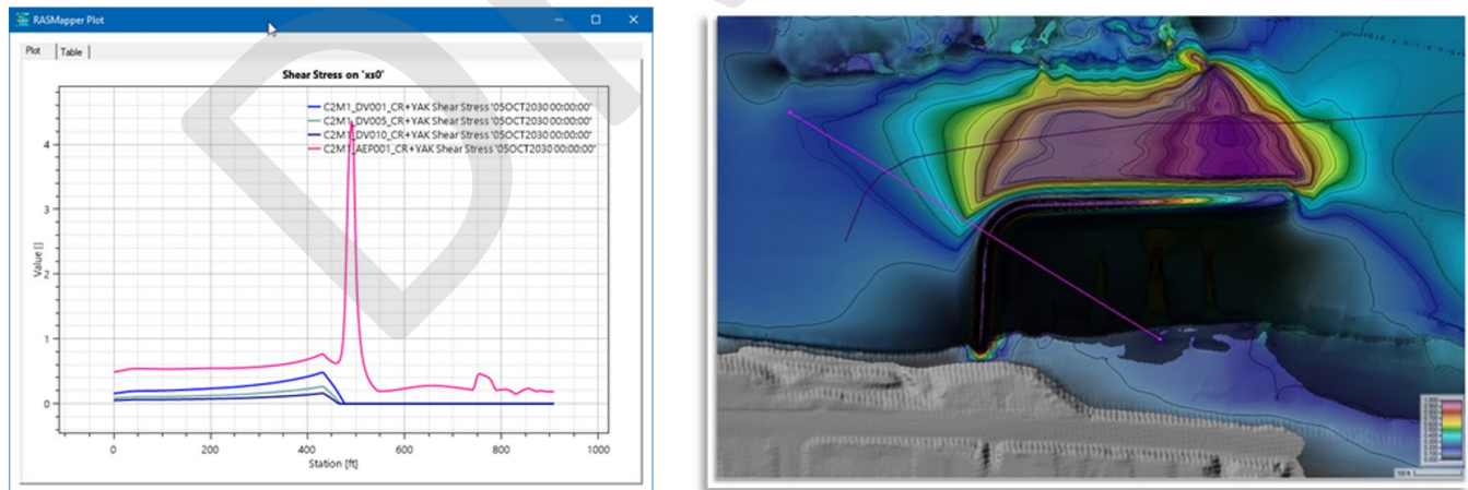
Figure 4-13. Shear Stress Cross-Section across upstream side of M1: Levee Marina Barrier
