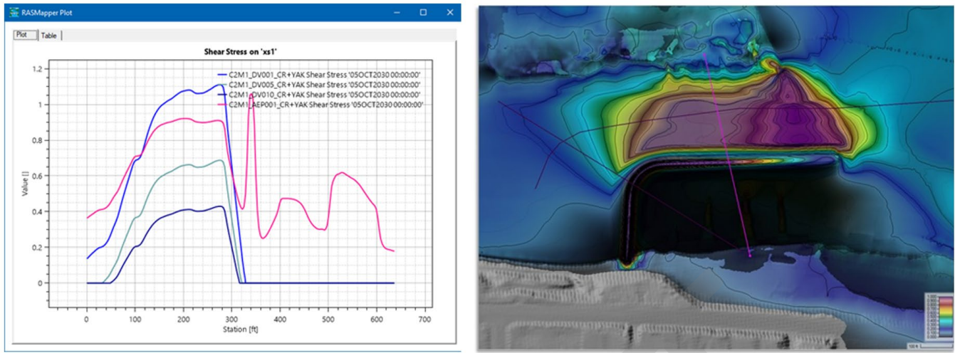
Figure 4-14. Shear Stress Cross-Section across M1: Levee Marina Barrier
