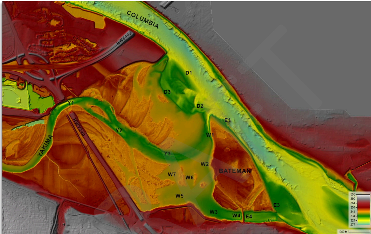
Figure 3-4. Yakima Delta study area monitoring locations from 2021 SRP used to query model results.
