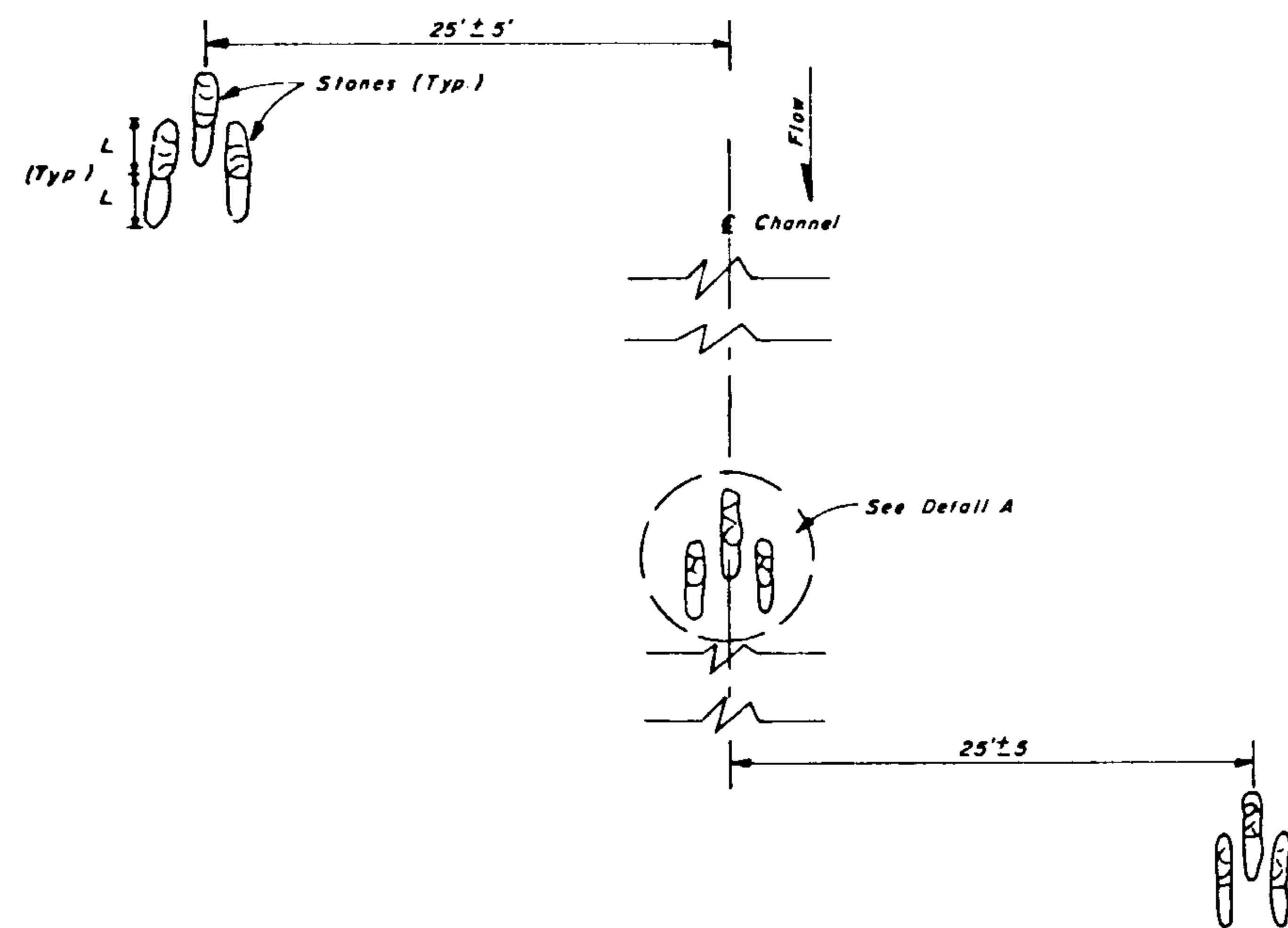
DETAIL PLAN NOT TO SCALE
